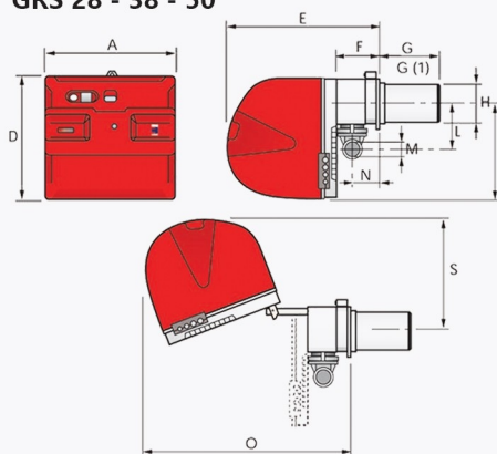
GRS 28 - 38 - 50
