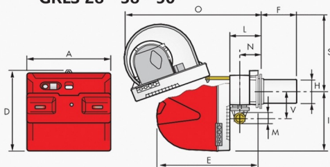
GRLS 28 - 38 - 50
