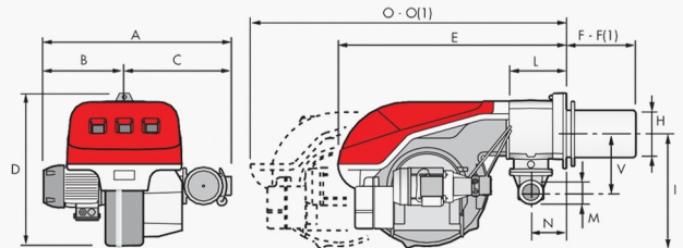
GRLS 70 - 100 - 130
